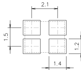
Reference Footprint
